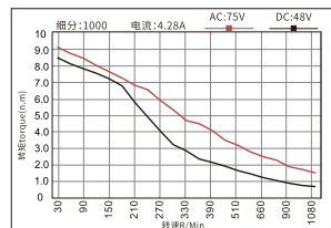
电机型号:YK86HB156-06A
